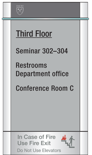
directories
